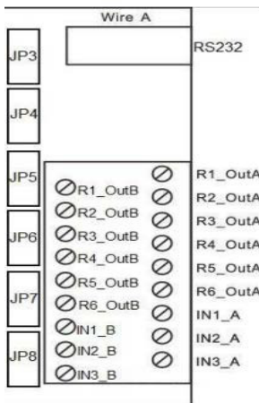
Pin outs
