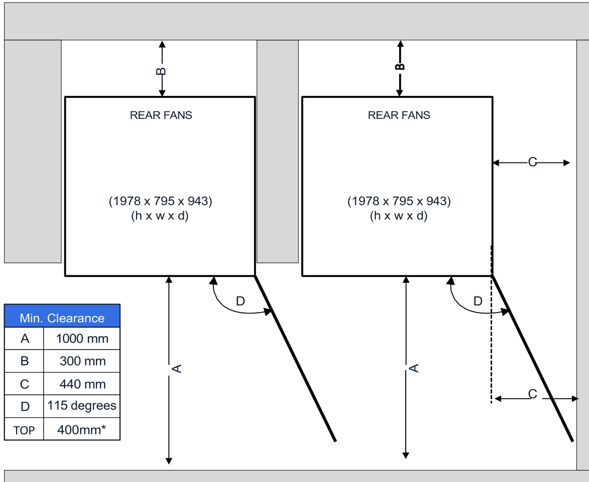
Figure 7 Clearances for a Rehiko PW 9250DPA stand-alone cabinet
