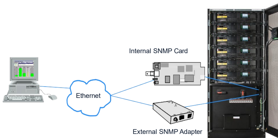
Figure 5 SNMP Connection
