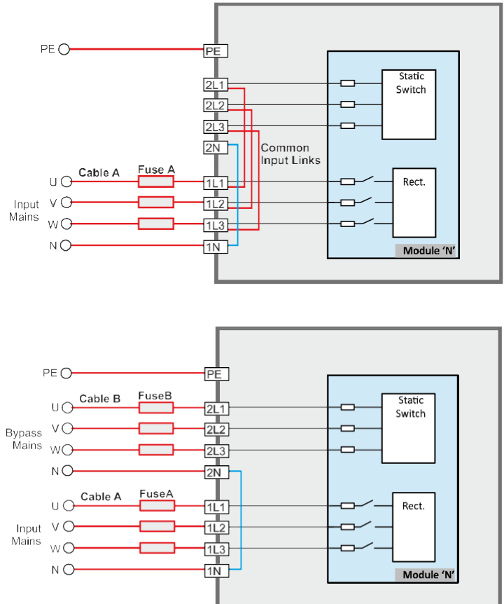
Figure 9 Single and Dual feed input supply options
