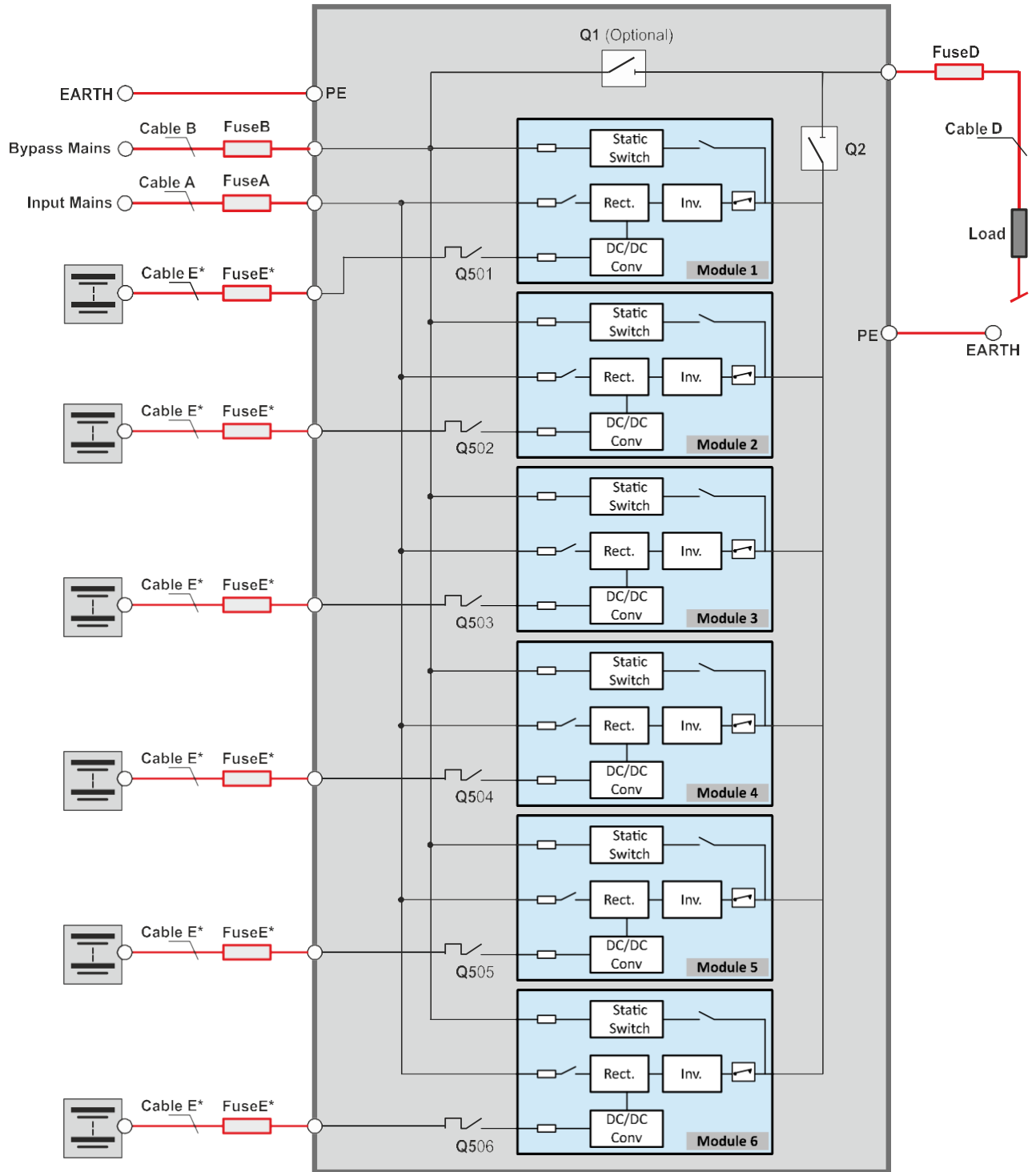
Figure 14 UPS cabinet cabling details for a dual-feed input and separate batteries
