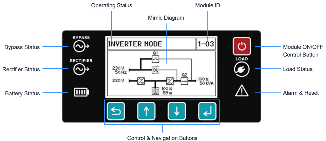
Figure 2 Module Control Panel
