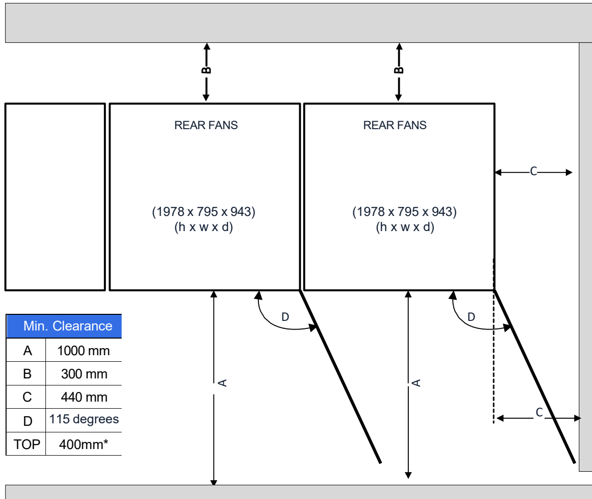
Figure 8 Clearances for a Rehiko PW 9250DPA parallel-cabinet installation
